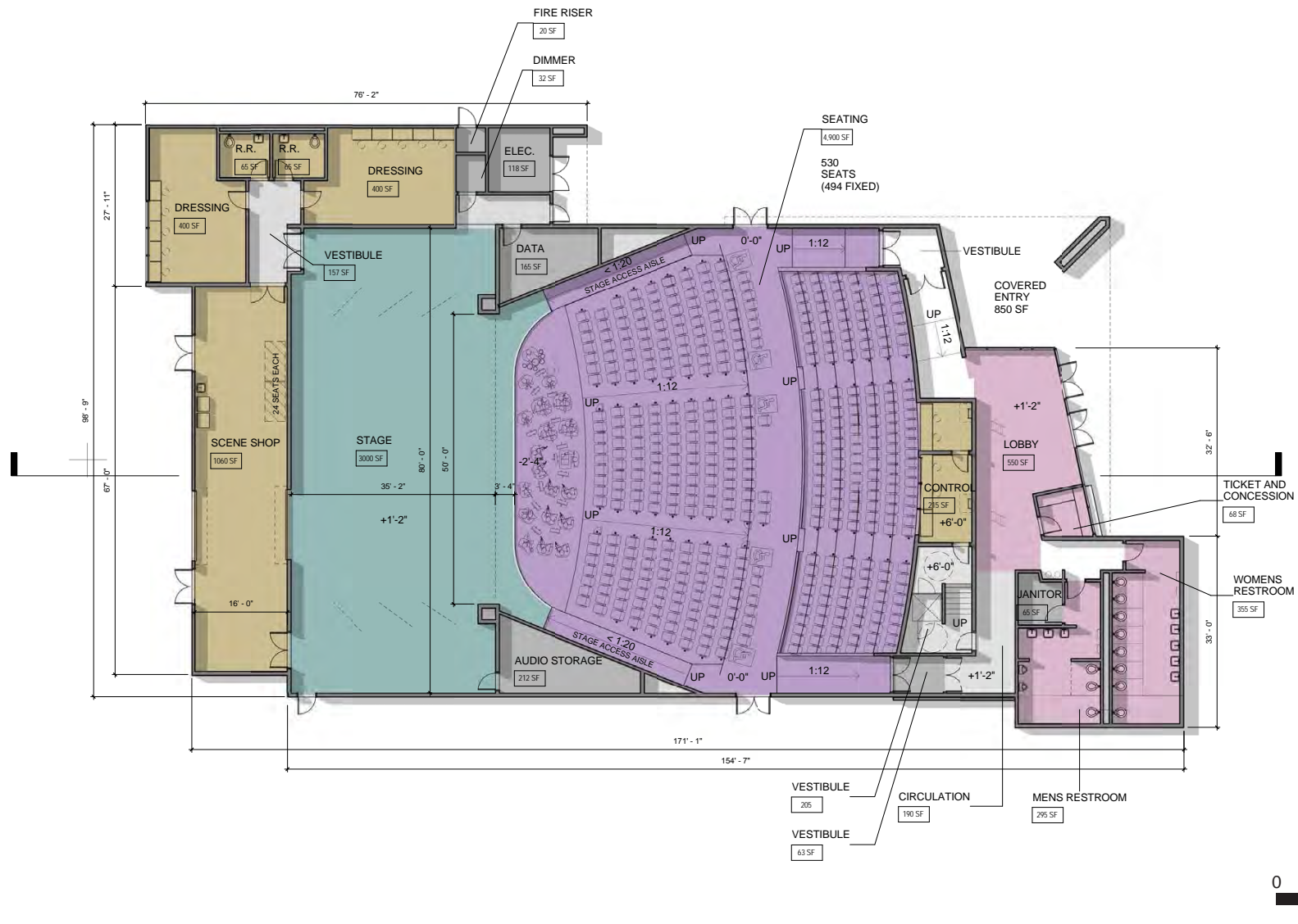
Figure 6 - Auditorium Floor Plan
