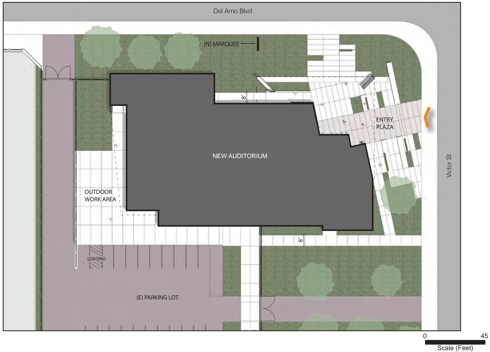
Figure 5 - West High School Auditorium Site Plan
